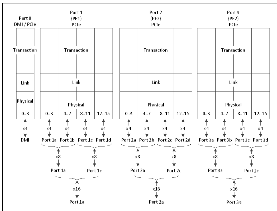
Figure 1-3. PCI Express* Lane Partitioning and Direct Media Interface Generation 3 (DMI3) with 48 PCIe lane
